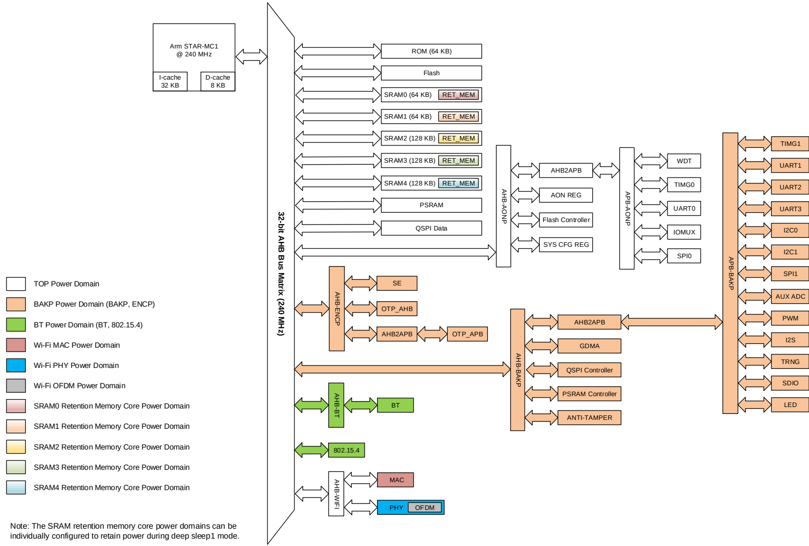
Figure 2-2 BK7239N Bus Interconnect
