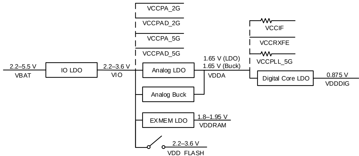
Figure 4-6 Internal Power Distribution
