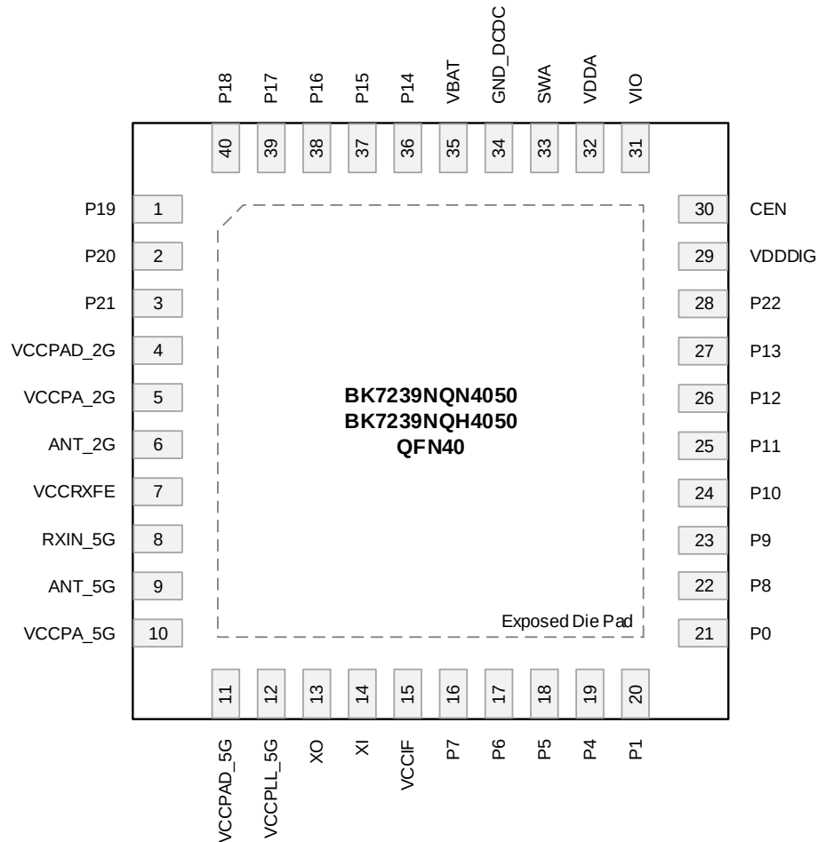
Figure 3-2 BK7239NQN/H4050 QFN40 Pin Assignments
