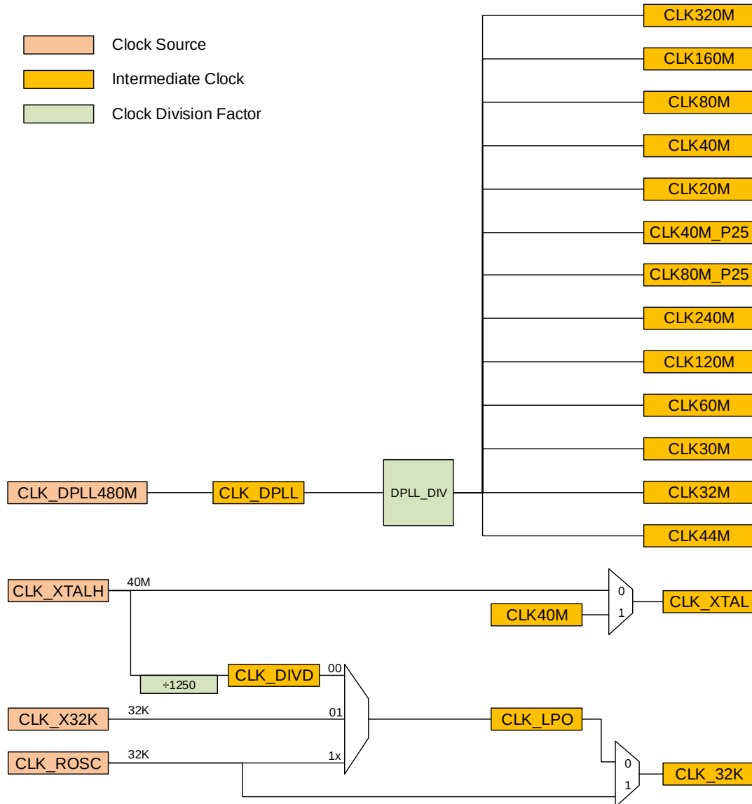
Figure 4-2 Clock Generation
