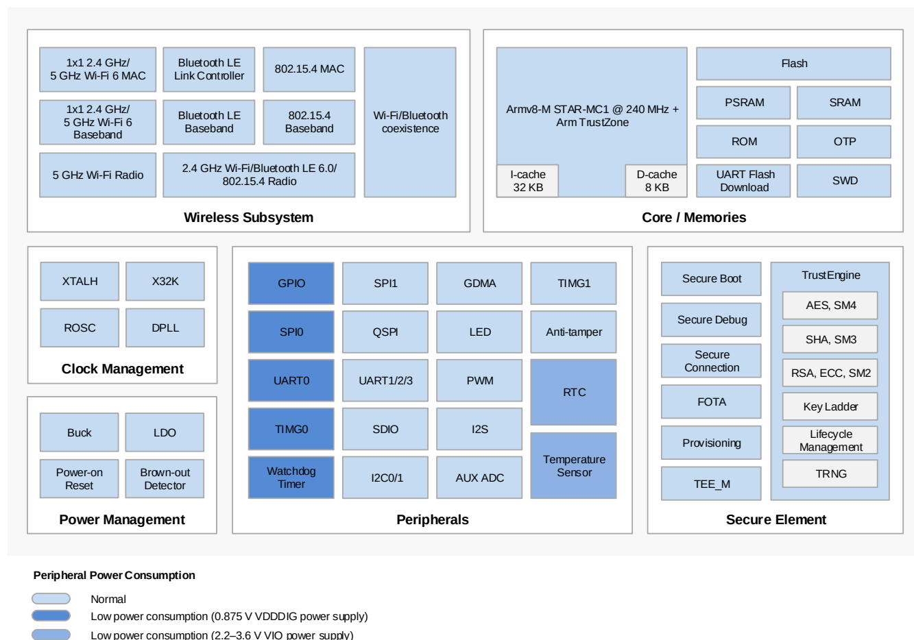
Figure 2-1 BK7239N Block Diagram
