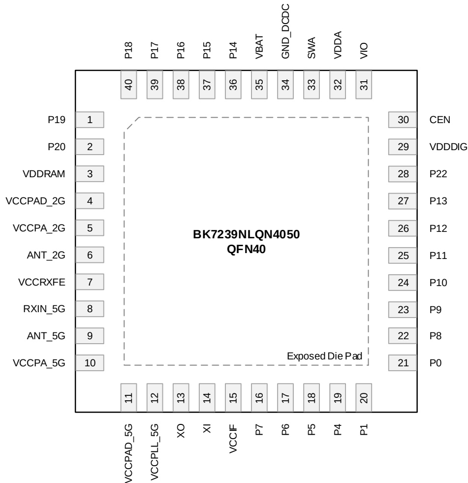
Figure 3-3 BK7239NLQN4050 QFN40 Pin Assignments
