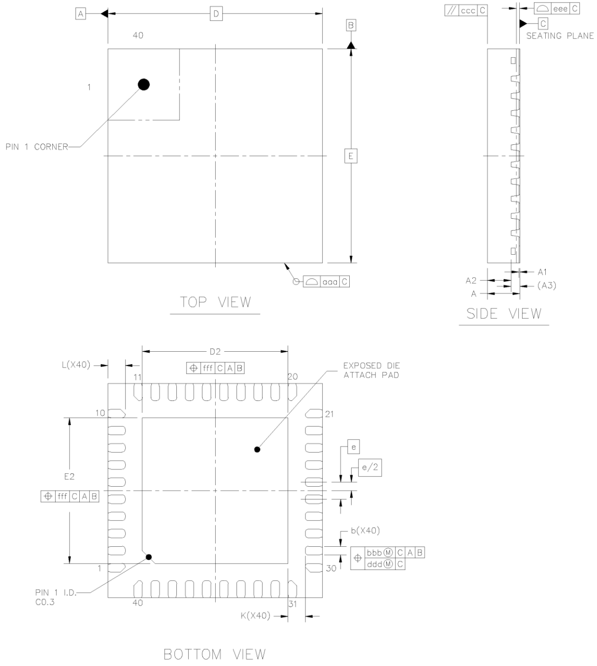
Figure 6-2 QFN40 5 x 5 x 0.75 mm Package Outline
